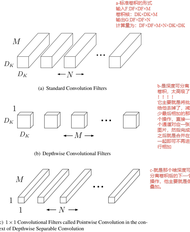
Figure 2. The standard convolutional filters in (a) are replaced by two layers: depthwise convolution in (b) and pointwise convolution in (c) to build a depthwise separable filter.
